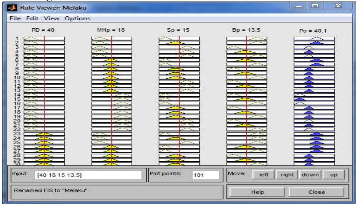
Fig 4.9 Rule viewer
