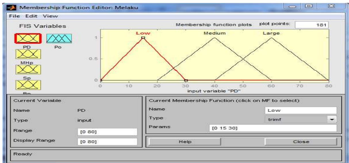
Fig 4.3 Membership function of power demand real time simulated version
