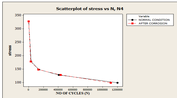
GRAPH 7 - Relation between Stress and No of cycles under Normal condition and after Corrosion of the specimens
