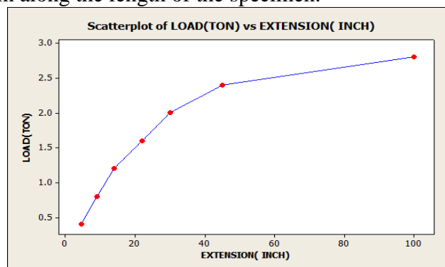
GRAPH 1 - Relation between LOAD (TON) and EXTENSION (INCH)
