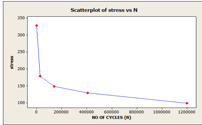
GRAPH 2 - Relation between Stress and No of cycles under Normal condition of the specimens
