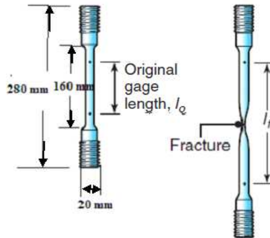
Figure. 10- Tensile test specimen dimension
