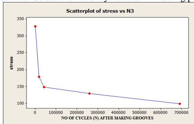
GRAPH 3 - Relation between Stress and No of cycles after Annealing process of the specimens
